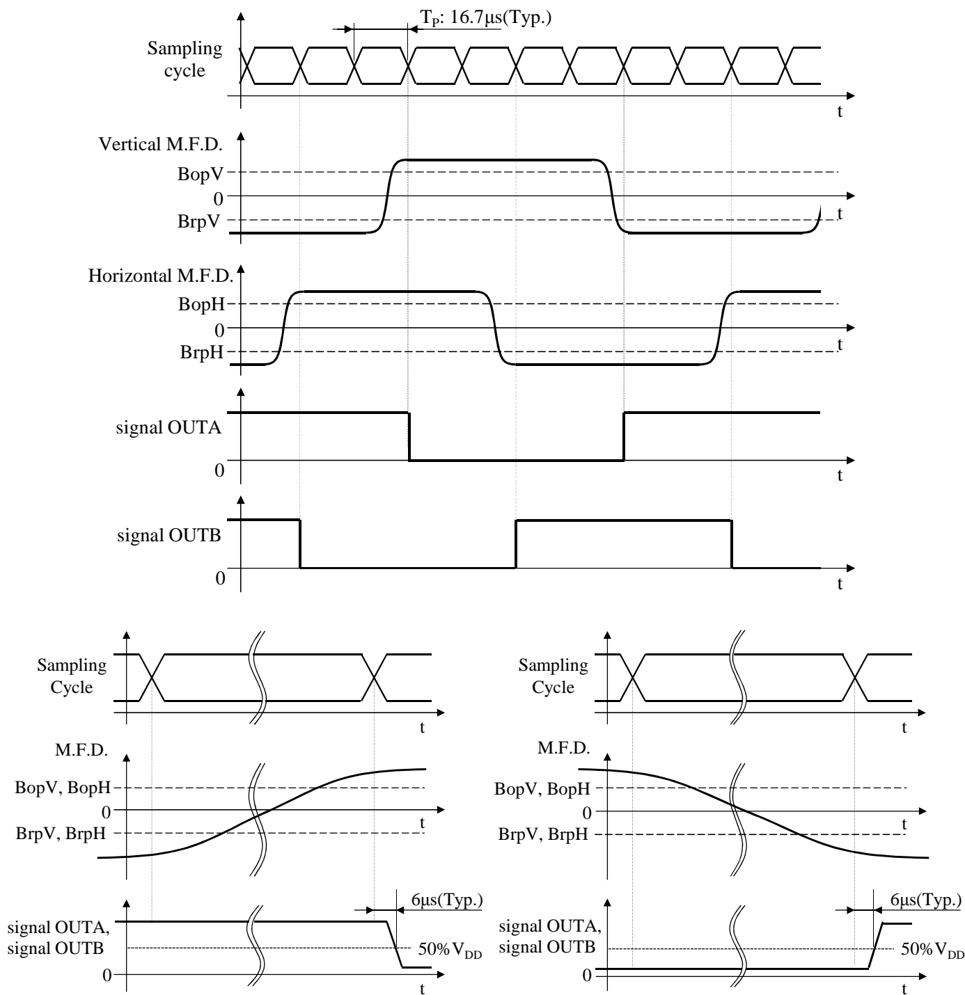
Figure 4. Timing diagram
