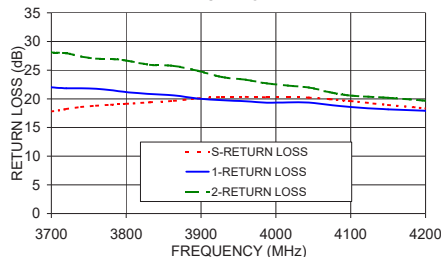
SCN-2-45 RETURN LOSS
