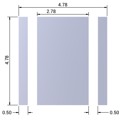
3-V and 6-V PCB Footprint Depending on Vf Class (Thermal pad is electrically isolated)
