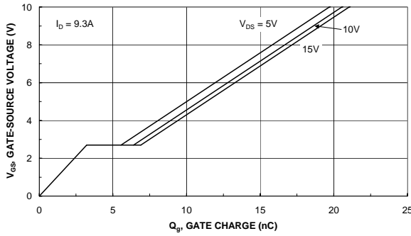
Figure 7. Gate-Charge Characteristics
