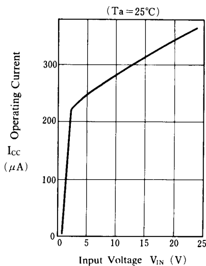
Operating Current
