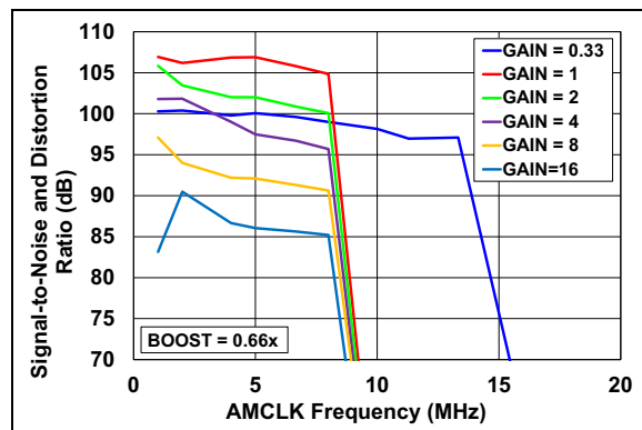
FIGURE 2-36: SINAD vs. AMCLK (BOOST = 0.66X).
