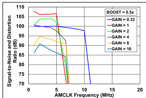
FIGURE 2-35: SINAD vs. AMCLK (BOOST = 0.5X).
