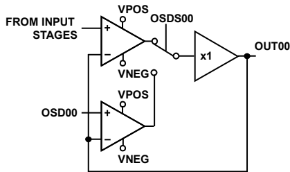
Figure 19. Conceptual Diagram of Single Output Channel, G = +1 (ADV3202)
