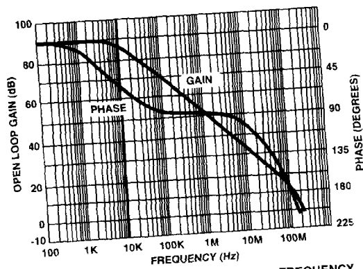
FIGURE 16. OPEN LOOP GAIN/PHASE vs FREQUENCY
