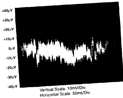
FIGURE 13. BROADBAND NOISE (0.1Hz TO 1MHz) Vertical Scale: 10mV/Div. Horizontal Scale: 50ms/Div.
