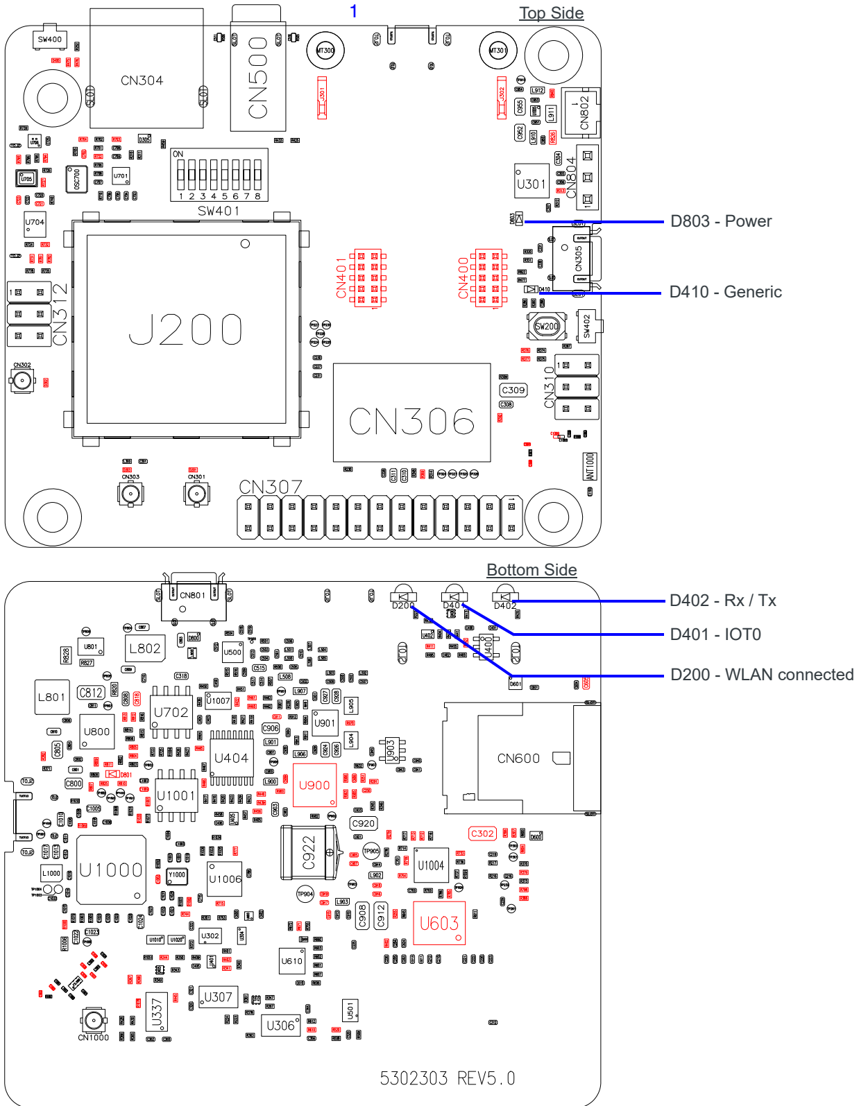
Figure 3-22: LED Indicators
