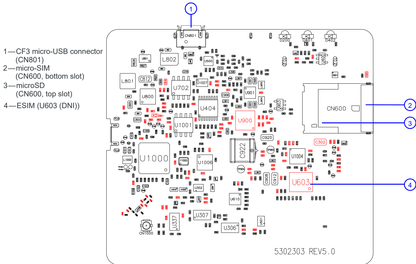
Figure 3-26: mangOH Red Assembly - Bottom Side Connectors
