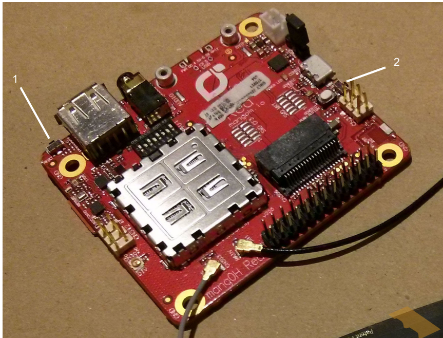
Figure 3-23: Reset Switches
