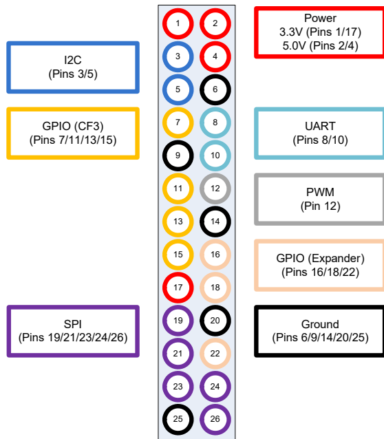
Figure 3-17: Raspberry Pi Connector Signal Groups
