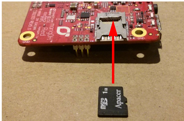
Figure 3-12: microSD—Inserting
