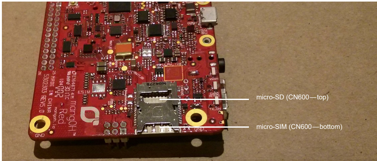
Figure 3-9: SIM Connector and micro-SD Locations
