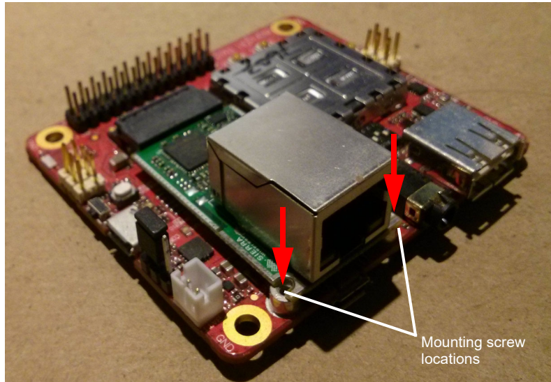
Figure 3-15: IoT Expansion Card Inserted
