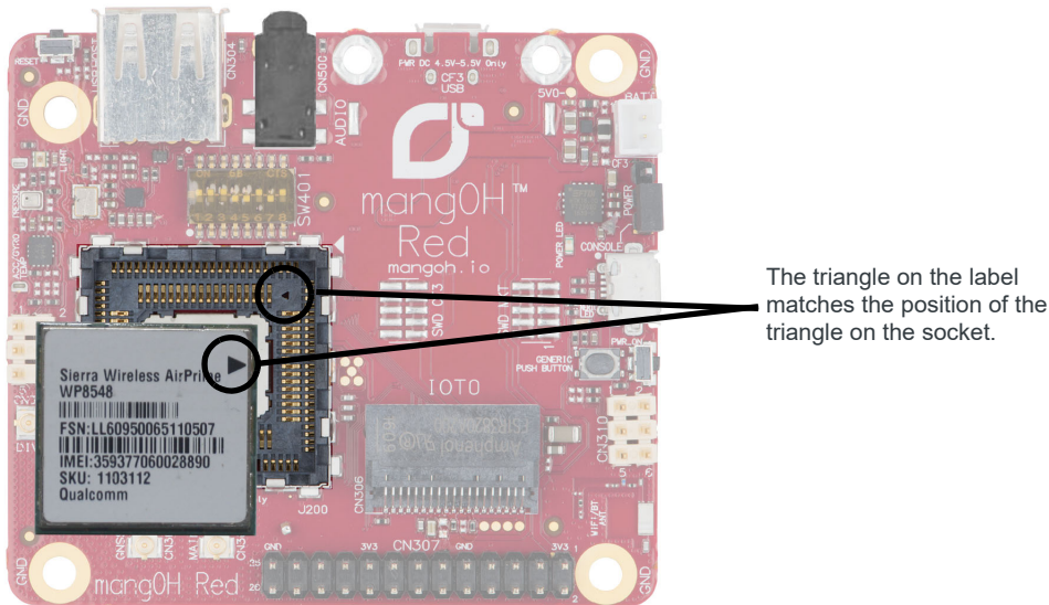
Figure 3-1: mangOH Red—Module Insertion
