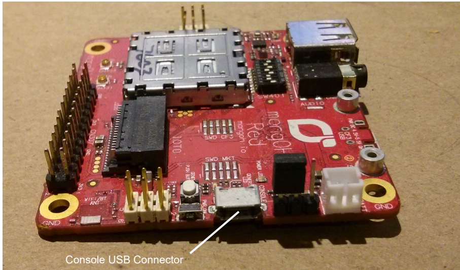
Figure 3-20: Console USB Output Connection
