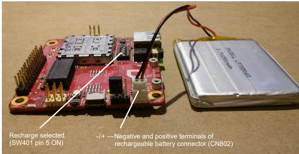
Figure 3-7: mangOH Red With Rechargeable Battery Connected
