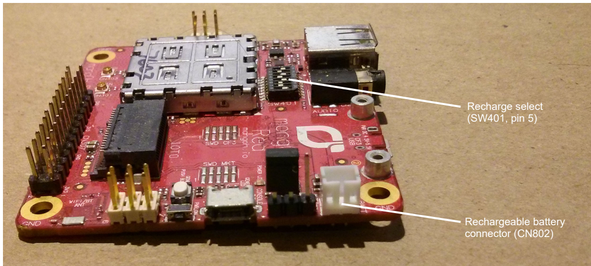
Figure 3-6: Battery Backup Connector
