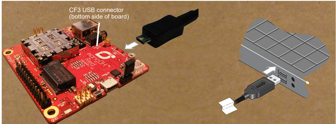
Figure 2-5: Connecting Power to the mangOH Red
