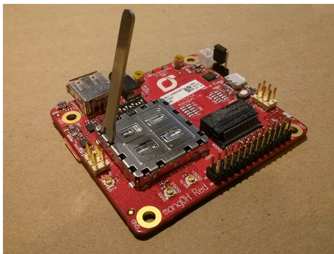
Figure 3-3: mangOH Red—Module Removal
