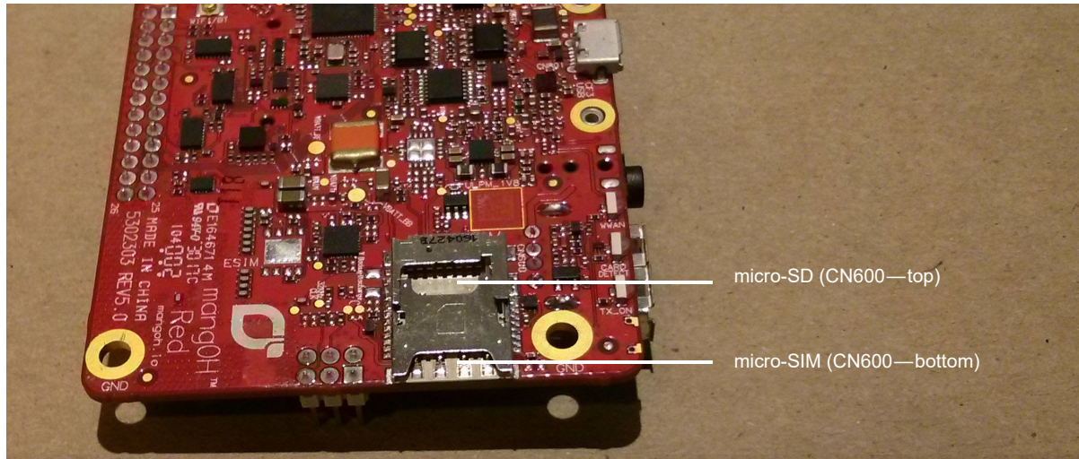
Figure 3-11: SIM Connector and microSD Locations
