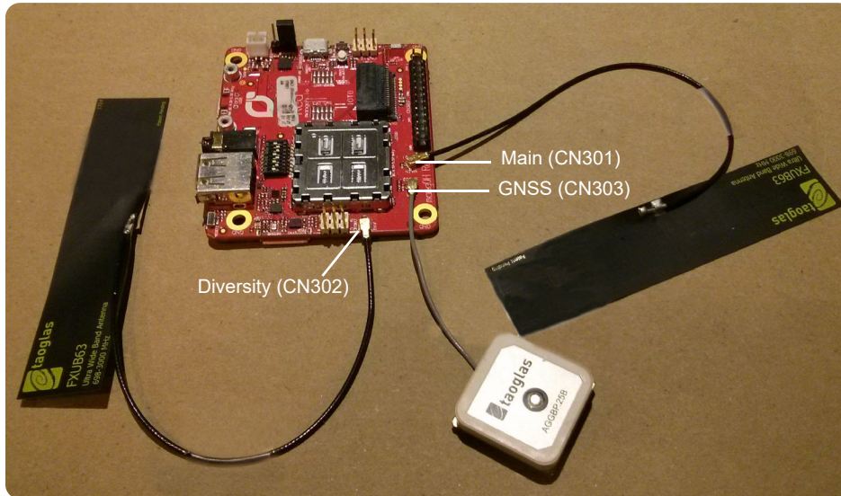
Figure 3-8: Antenna Connector Locations
