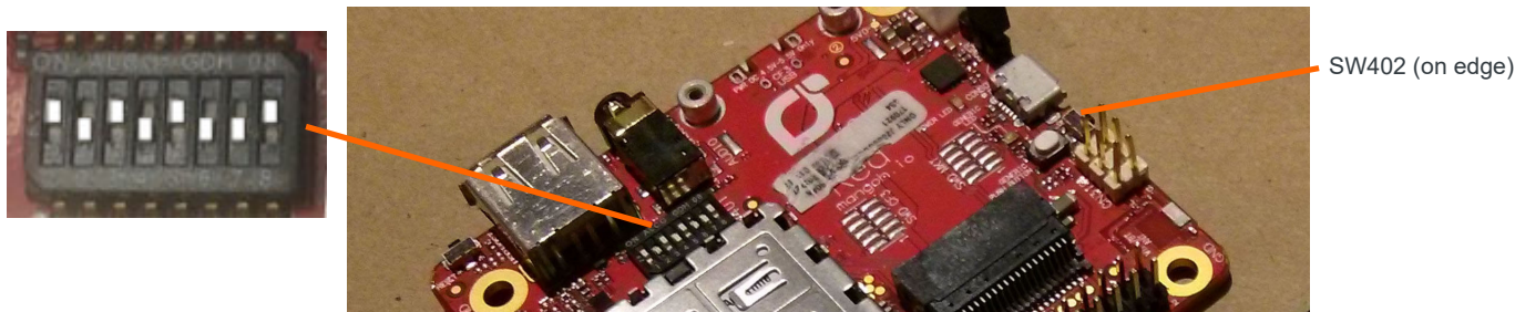
Figure 2-4: SW401 Dipswitch Recommended Settings
