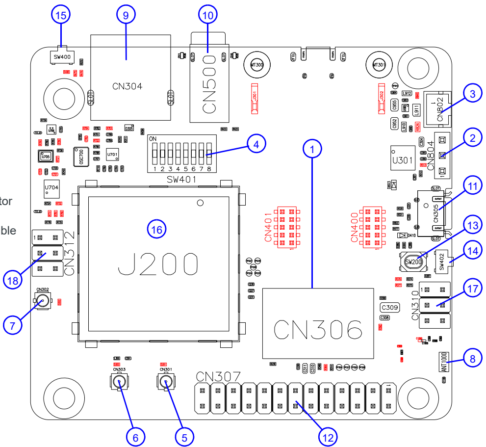
Figure 3-25: mangOH Red Assembly— Top Side Switches/Connectors
