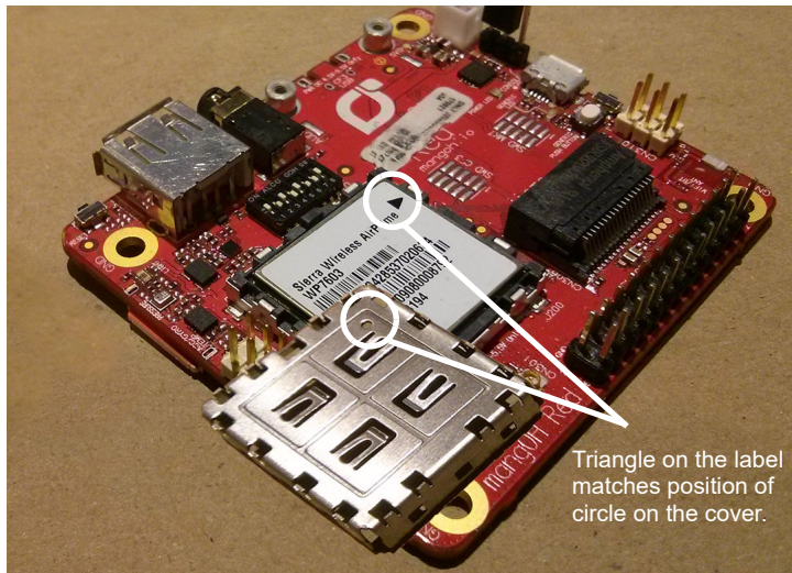
Figure 3-2: mangOH Red—Module Cover Attachment
