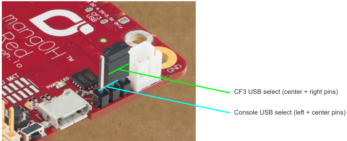
Figure 3-5: USB Power Supply Selection
