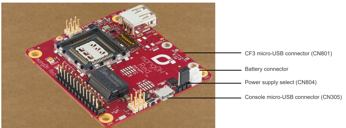
Figure 3-4: Power Supply Connectors/Selector
