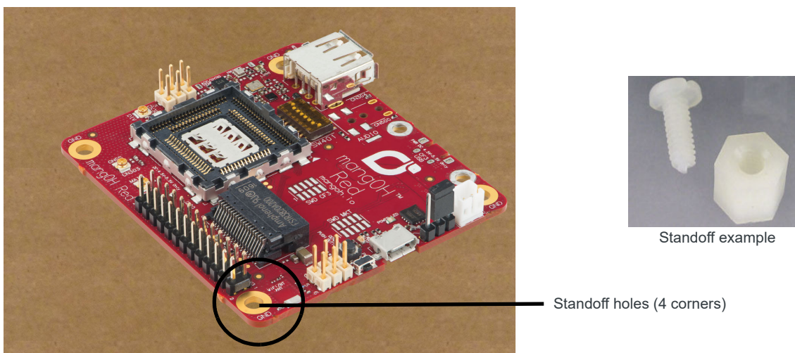
Figure 2-2: Module Standoff Placement
