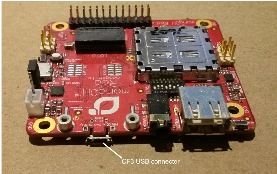
Figure 3-21: CF3 USB Connector
