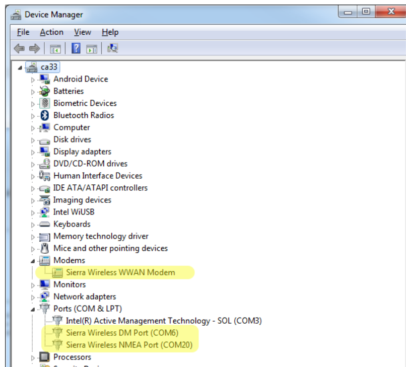
Figure 4-1: Windows Device Manager
