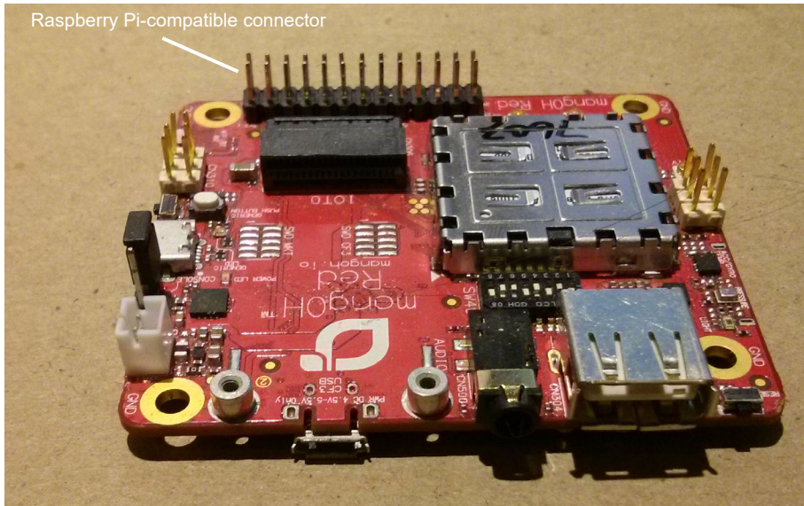
Figure 3-16: Raspberry Pi Connector
