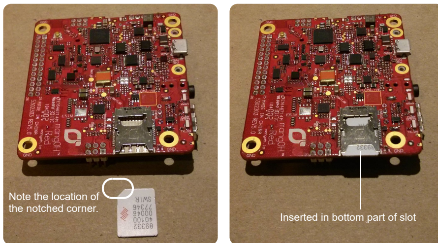
Figure 3-10: SIM Insertion
