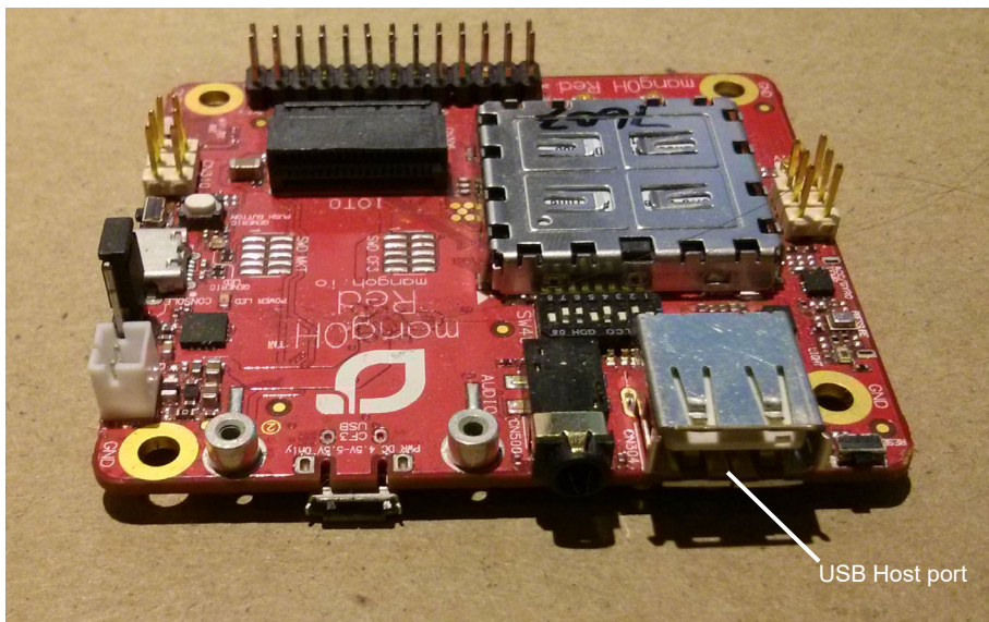
Figure 3-19: USB Host Port
