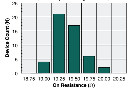
Typical On-Resistance Distribution (N=50, I_F=5mA , I_L=120mA )
