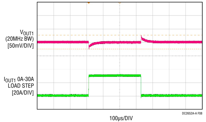
Figure 8. V OUT1 Load Transient Response at V IN = 12V, V OUT1 = 1.0V
