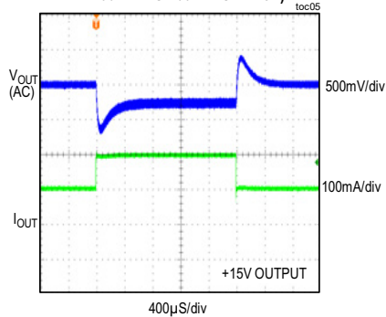
LOAD TRANSIENT RESPONSE (LOAD CURRENT FROM 100mA TO 200mA ON +15V)
