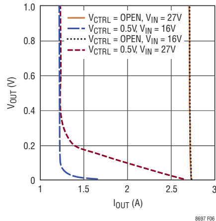
Figure 6. Output Current Regulation vs V_{OUT} at f_{sw} = 2MHz , R_{SENSE} = 18m\Omega
