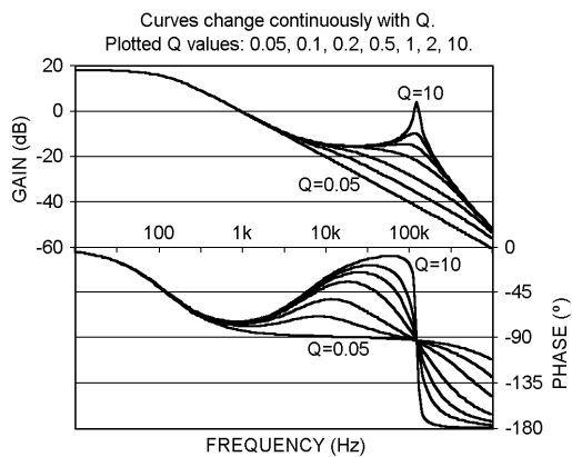
FIGURE 15. How Control-Output Transfer Function Changes with Q Values
