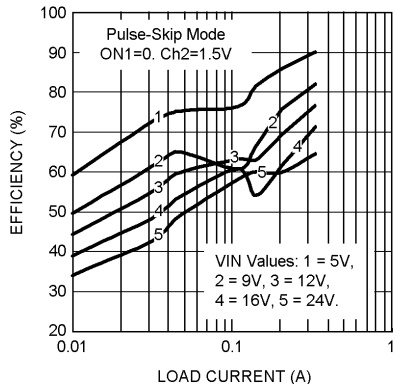
Efficiency vs Load Current (Ch2, Typical Application, FPWM = 1)
