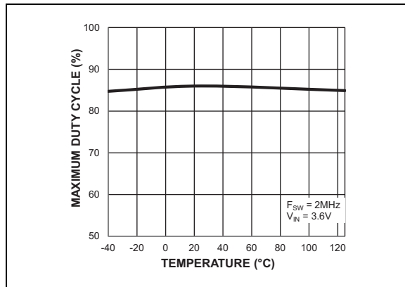
FIGURE 2-5: Maximum Duty Cycle vs. Temperature.
