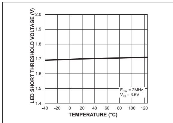
FIGURE 2-6: LED Short Threshold Voltage vs. Temperature.
