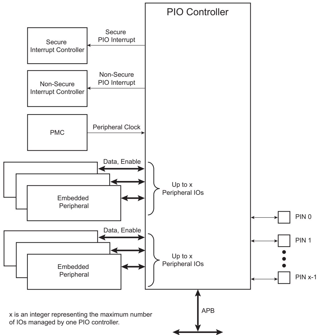
Figure 28-1: Block Diagram
