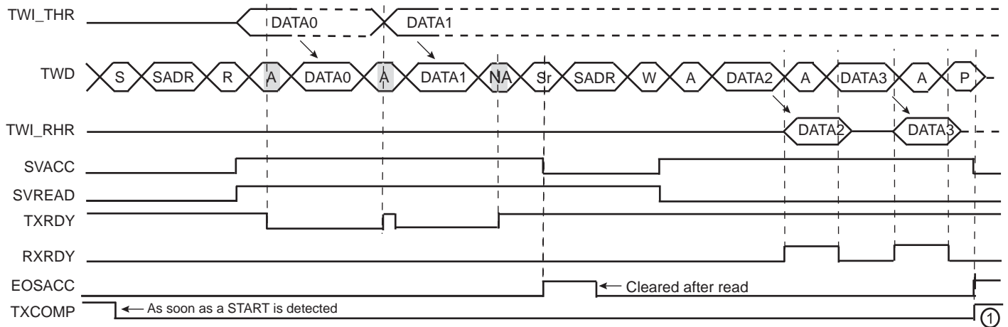
Figure 40-27: Repeated Start + Reversal from Read to Write Mode
