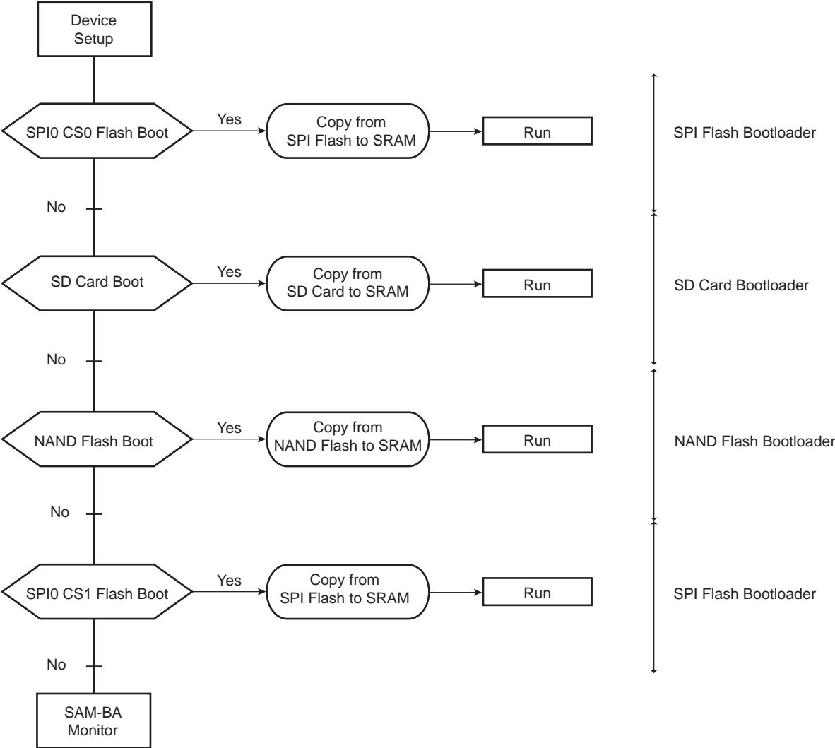
Figure 12-2: NVM Bootloader Sequence Diagram
