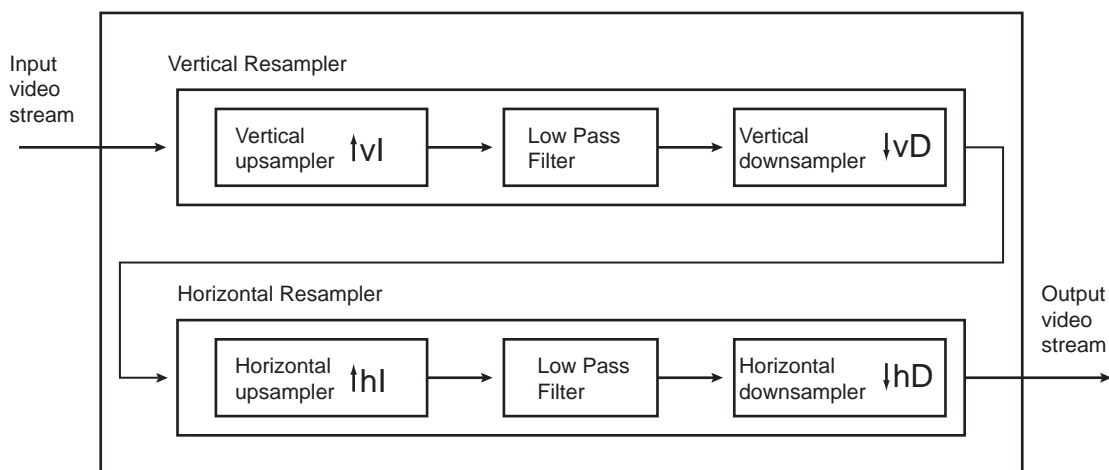
Figure 32-6: Video Resampler Architecture
