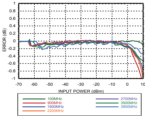
Figure 16. Reading Error for LTE wrt CW Response @ +25 °C
