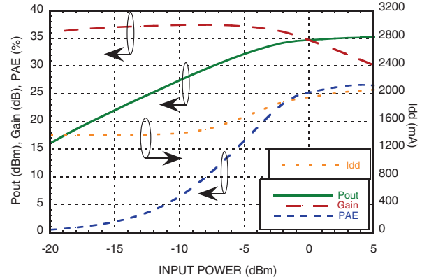
Power Compression @ 9.5 GHz
