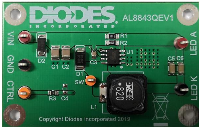
Figure 1: Top View
