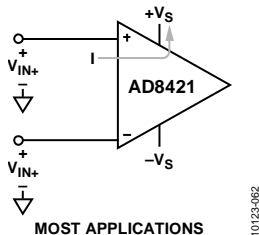
Figure 67. Typical Application; No Input Protection Required
