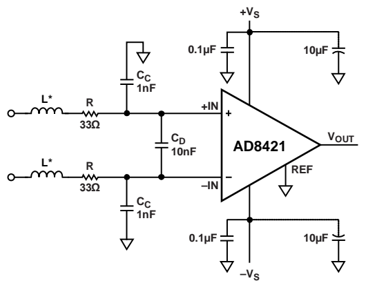
Figure 69. RFI Suppression
