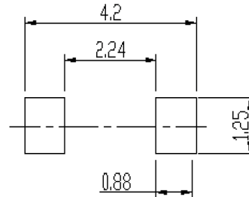
Soldering footprint
