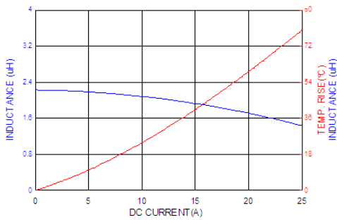
ASPIAIG-F7030-2R2
