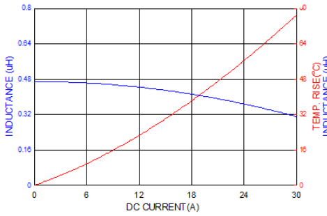
ASPIAIG-F7020-R47
