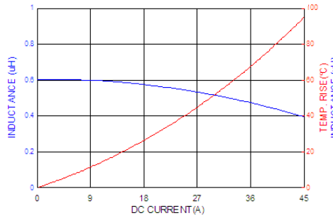
ASPIAIG-F7030-R60
