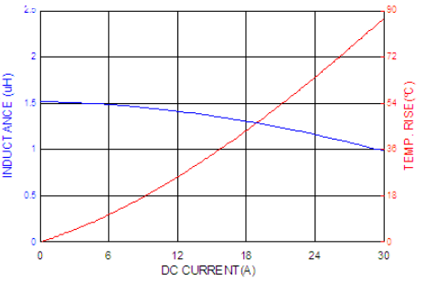
ASPIAIG-F7030-1R5
