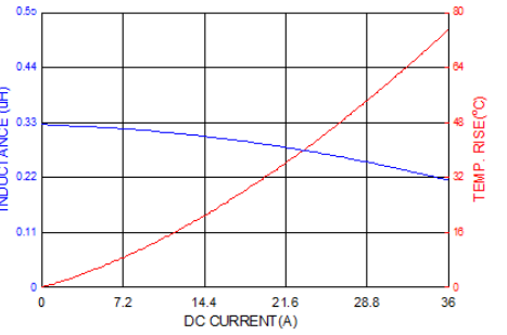
ASPIAIG-F7020-R33
