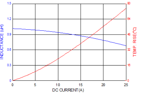
ASPIAIG-F7020-1R0
