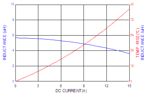
ASPIAIG-F7030-5R6
