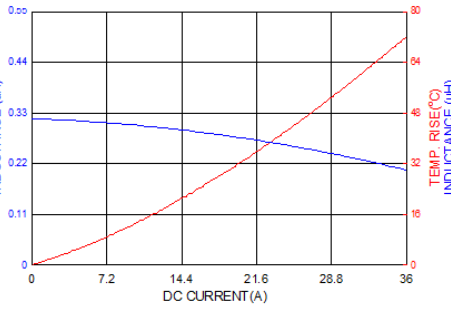
ASPIAIG-F7020-R31
