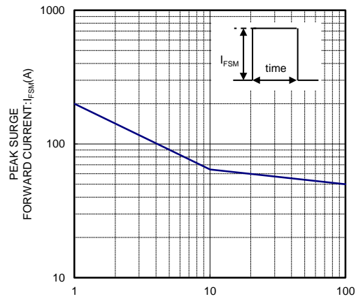
I_{FSM} TIME CHARACTERISTICS
