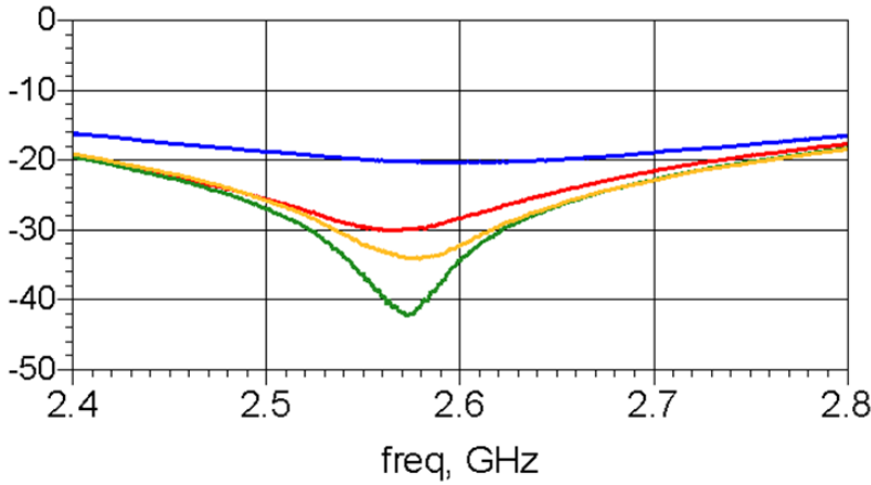
Figure 9.1 S11 (IRL) vs Freq
