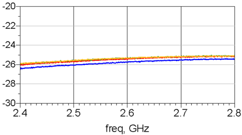
Figure 9.3 S12 (Rev Iso) vs Freq
