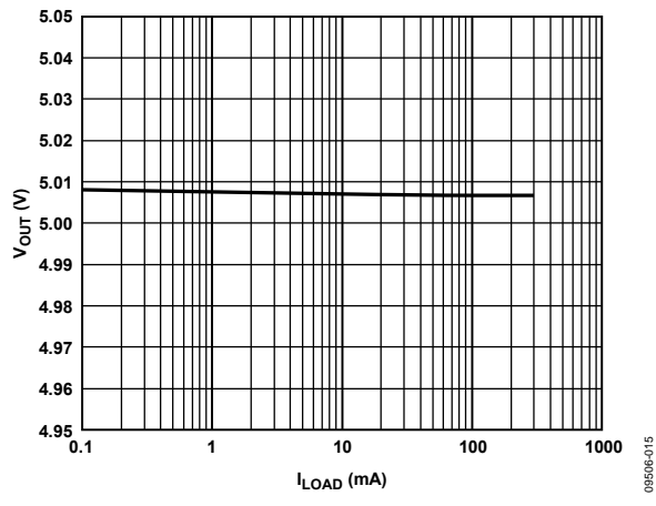
Figure 16. Output Voltage vs. Load Current, V_{OUT} = 5 V
