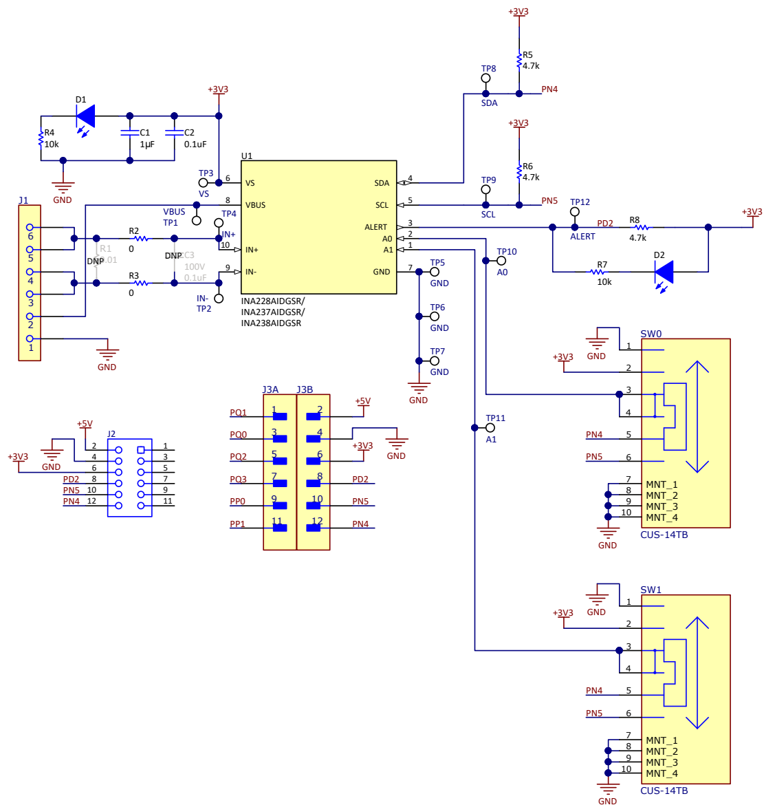
Figure 6-1. SENS063 Schematic
