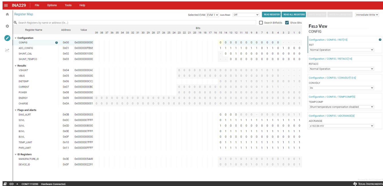
Figure 4-11. GUI Registers Tab
