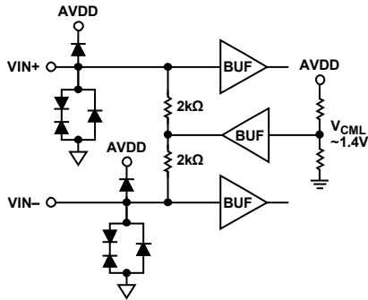
Figure 7. Analog Inputs ( V_{CM} = \sim 1.4V )
