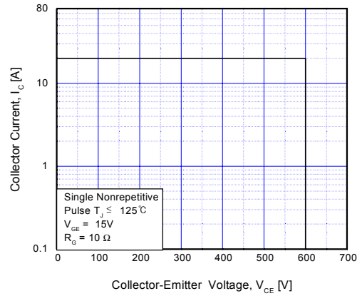
Fig 14. RBSOA Characteristics
