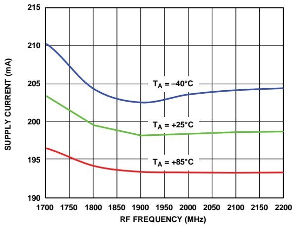
Figure 46. Supply Current vs. RF Frequency at 3.3 V
