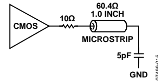
Figure 25. Series Termination of CMOS Output
