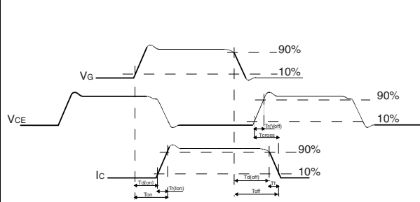
Figure 31. Switching waveform
