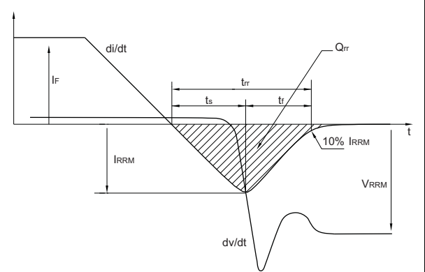
Figure 32. Diode recovery time waveform
