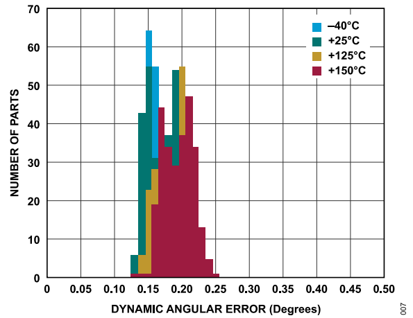
Figure 7. Dynamic Angular Error Histogram
