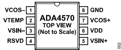
Figure 2. Pin Configuration
