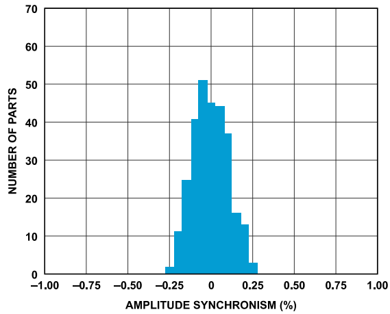
Figure 10. Amplitude Synchronism Histogram
