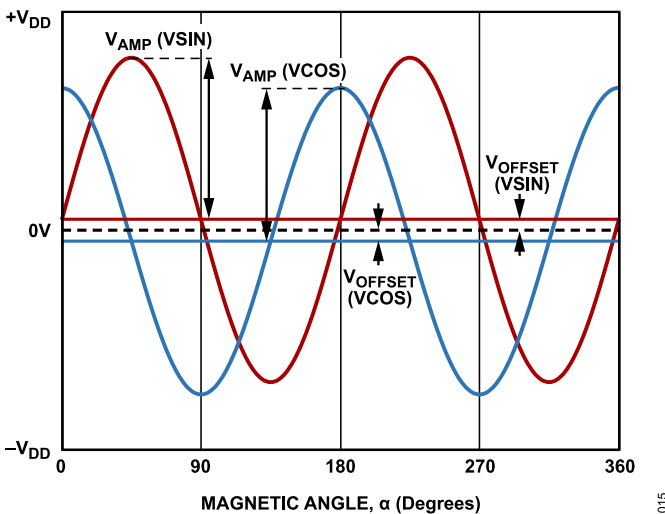
Figure 15. Differential Output Voltage Range
