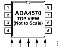
Figure 19. Direction of Homogeneous Magnetic Field for \alpha = 0^\circ
