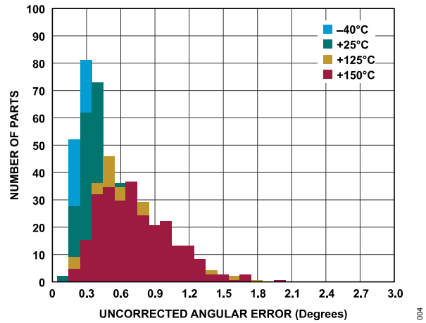
Figure 4. Uncorrected Angular Error Histogram
