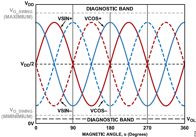
Figure 14. Single-Ended Output Voltage Range
