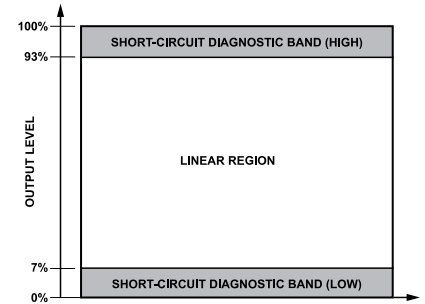
Figure 20. Short-Circuit Diagnostic Band
