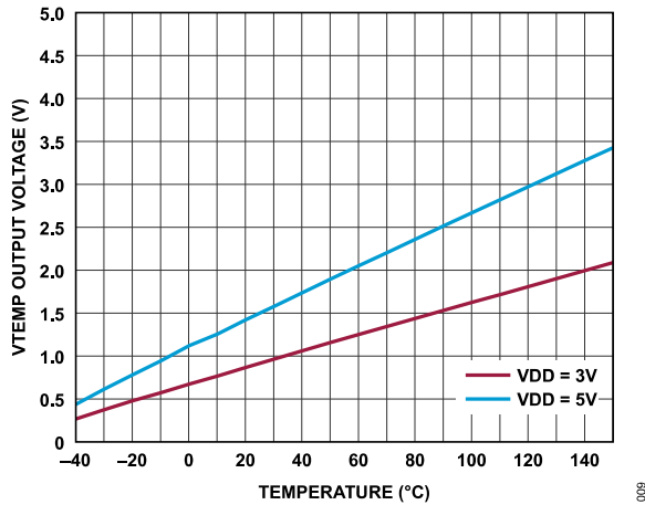
Figure 9. VTEMP Output Voltage vs. Temperature
