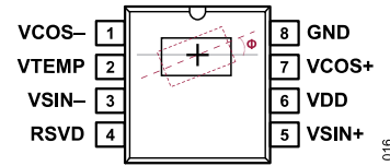
Figure 16. Sensor Alignment in Package
