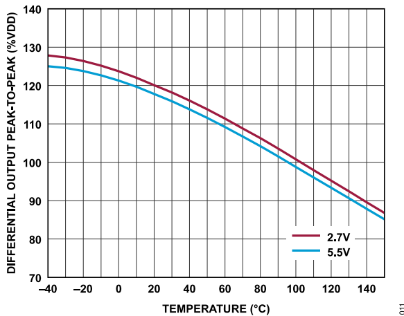
Figure 11. Differential Output Peak-to-Peak vs. Temperature
