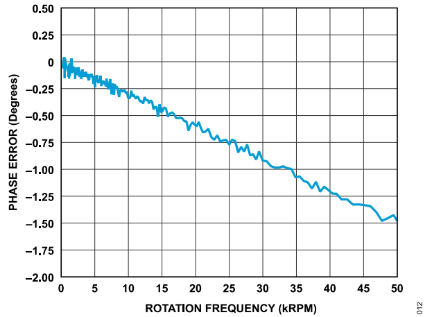
Figure 12. Phase Error vs. Mechanical RPM
