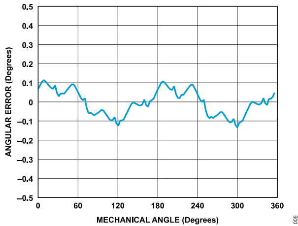
Figure 5. Angular Error vs. Mechanical Angle After Offset Correction
