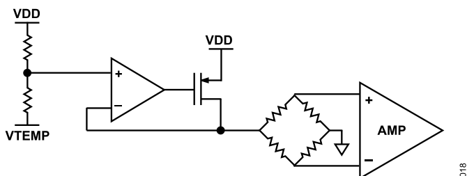
Figure 17. Temperature Compensated Bridge Driver
