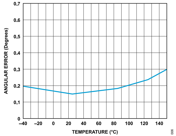
Figure 6. Single Point Calibration Angular Error vs. Temperature
