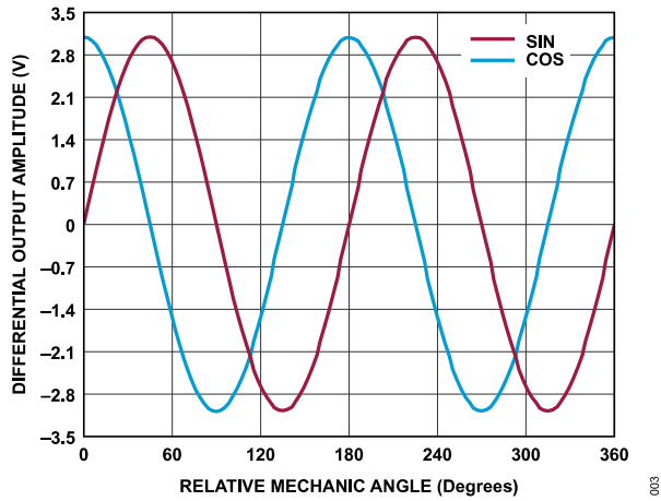
Figure 3. Differential Output Amplitude vs. Relative Mechanical Angle
