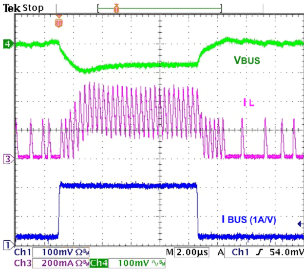
Figure 33. Load Transient, 20-200-20 mA I BUS , t RISE/FALL =100 ns
