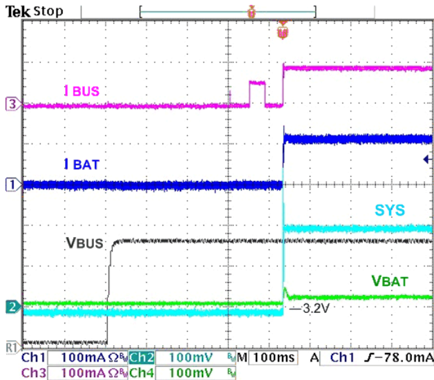
Figure 11. Charger Startup at V_{\text{BUS}} Plug-In, 100 mA I_{\text{BUSLIM}} , 3.2 V BAT , 100 Ω SYS Load
