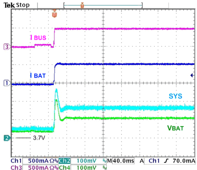
Figure 14. Charger Startup with HZ Bit Reset, 500 mA I_{\text{BUSLIM}} , 950 mA I_{\text{CHARGE}} , 50 Ω SYS Load
