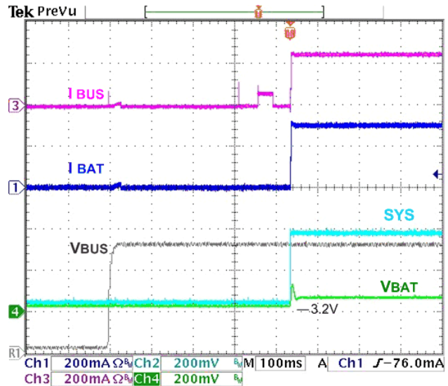
Figure 12. Charger Startup at V_{\text{BUS}} Plug-In, 500 mA I_{\text{BUSLIM}} , 3.2 V BAT , 100 Ω SYS Load
