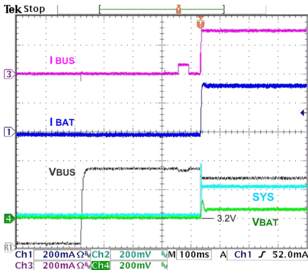
Figure 13. Charger Startup at V_{\text{BUS}} Plug-In Using 300 mA Current Limited Source, 500 mA I_{\text{BUSLIM}} , 3.2 V BAT , 50 Ω SYS Load
