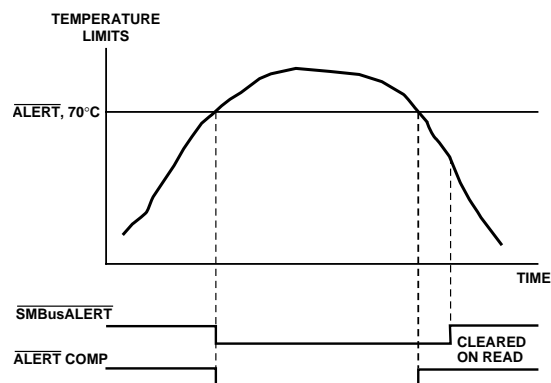
Figure 31. \overline{\text{ALERT}} Comparator and SMBusALERT Outputs
