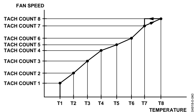
Figure 42. Programming the Look-Up Table in Linear Fan Speeds Mode
