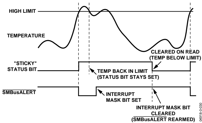
Figure 32. Handling SMBusALERT
