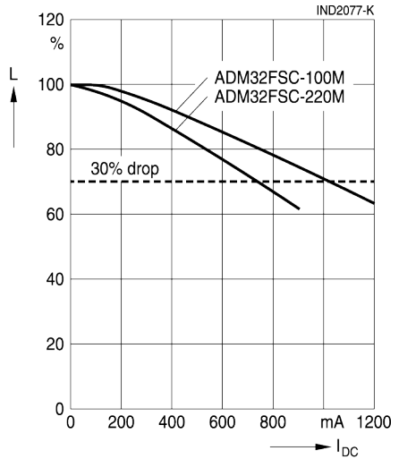
Saturation current I_{sat} (typical curves)
