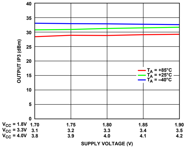
Figure 40. Output IP3 vs. Supply Voltage over Temperature
