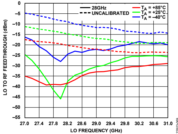
Figure 31. LO to RF Feethrough vs. LO Frequency, over Temperature, Not Calibrated and Calibrated with LO Frequency = 28 GHz at TA = 25°C, I/Q Mode
