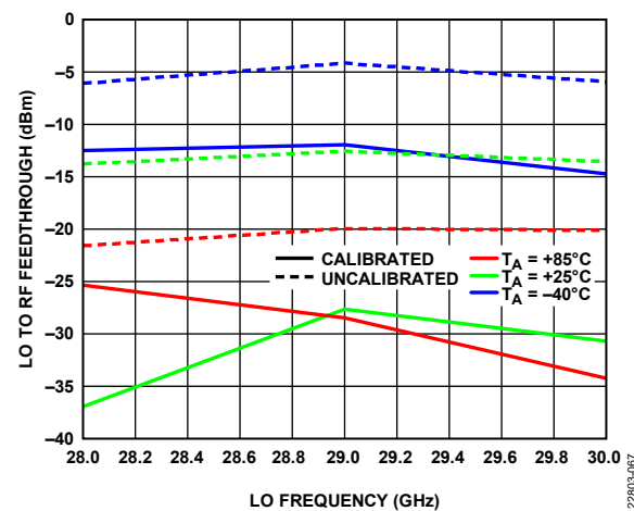
Figure 57. LO to RF Feedthrough vs. LO Frequency, Calibrated at T A = 25°C and Not Calibrated, over Temperature
