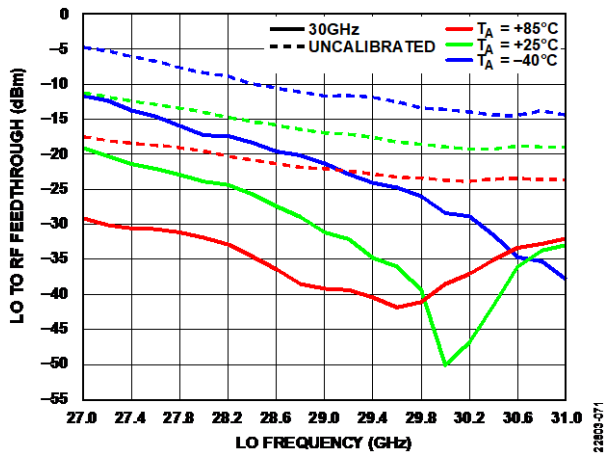
Figure 33. LO to RF Feethrough vs. LO Frequency, over Temperature, Not Calibrated and Calibrated with LO Frequency = 30 GHz at T A = 25°C, I/Q Mode
