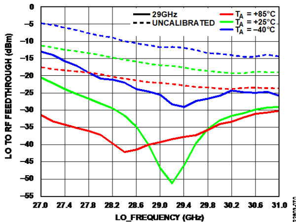
Figure 32. LO to RF Feethrough vs. LO Frequency, over Temperature, Not Calibrated and Calibrated with LO Frequency = 29 GHz at TA = 25°C, I/Q Mode
