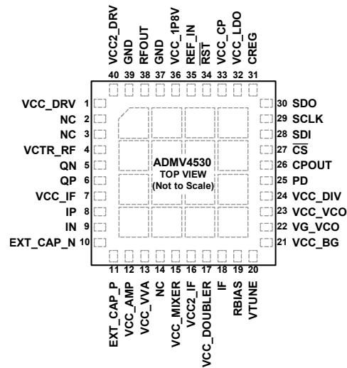
Figure 3. Pin Configuration
