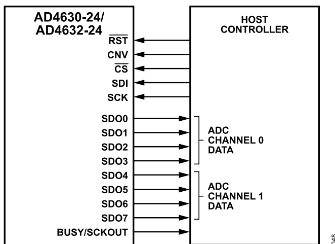
Figure 49. Multilane SPI
