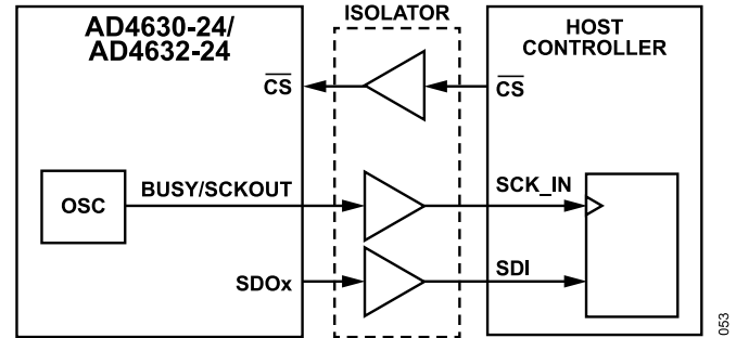
Figure 54. Host Clock Mode Signal Path Example
