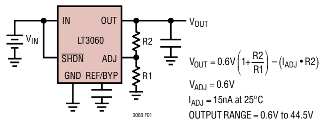
Figure 1. Adjustable Operation
