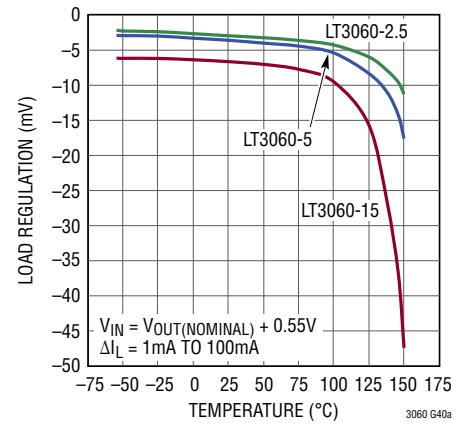
Load Regulation
