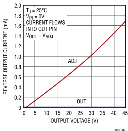
Figure 7. LT3060 Reverse Output Current
