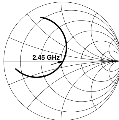
FREQUENCY (GHz): 2.3-2.6
