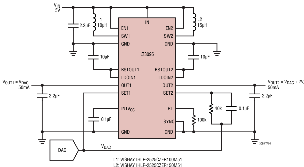
Programmable Outputs with Tracking
