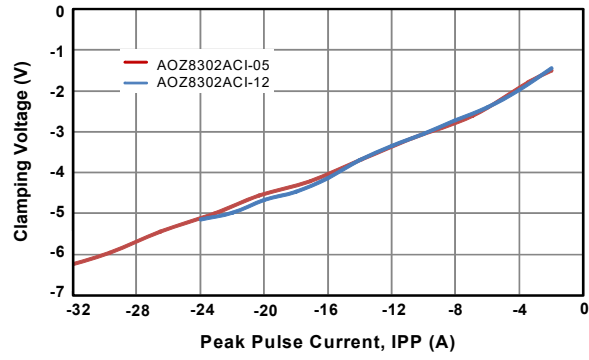
IEC61000-4-5 Surge 8/20 \mu s (Negative)
