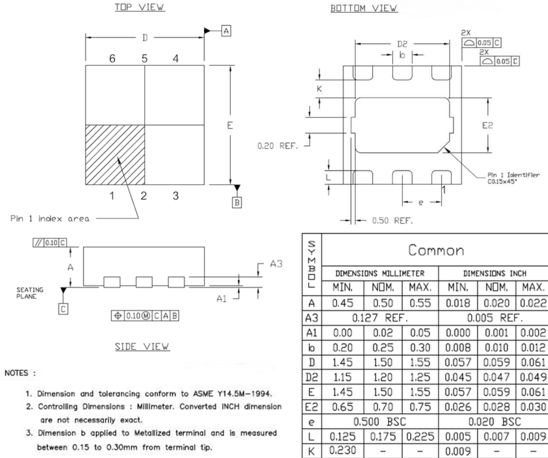
Figure 15 Package Outline Drawing
