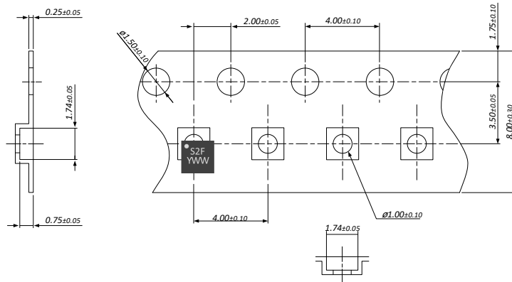
Figure 17 Tape & Reel
