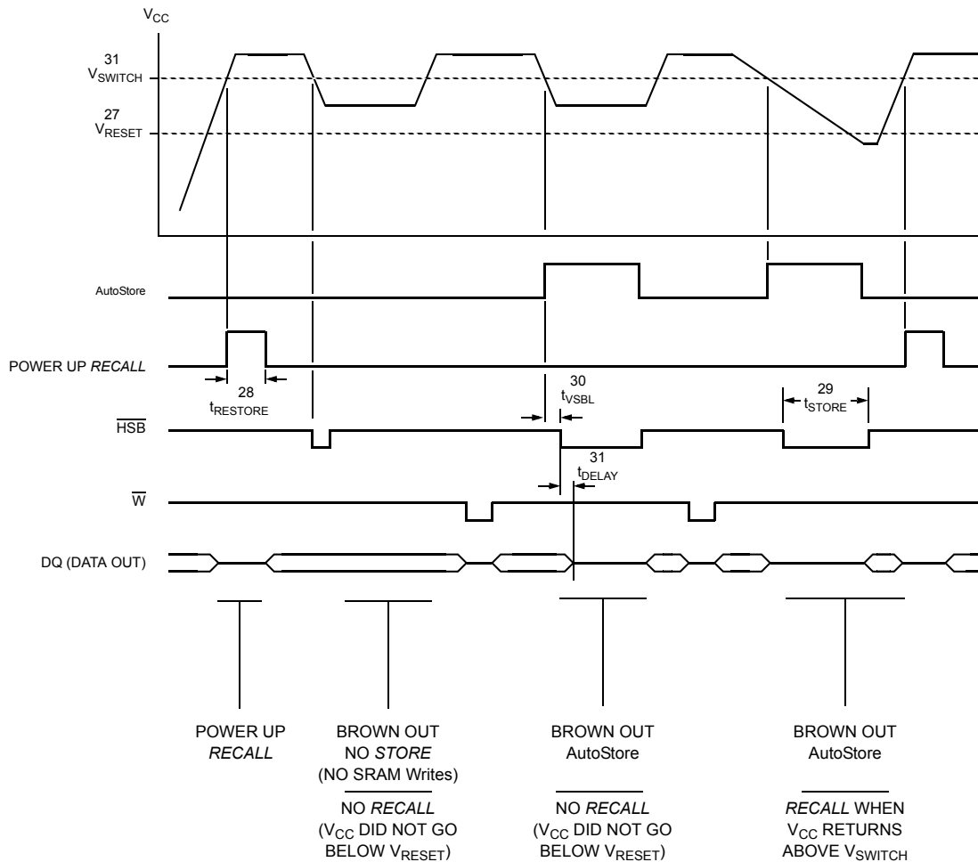
Figure 9. AutoStore/POWER UP RECALL
