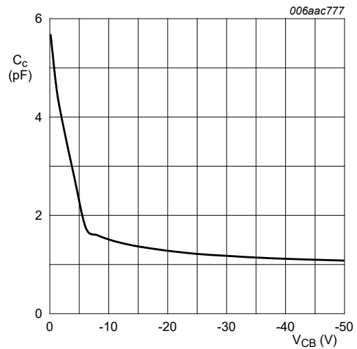
Fig. 15. PDTA114EQB: Collector capacitance as a function of collector-base voltage; typical values
