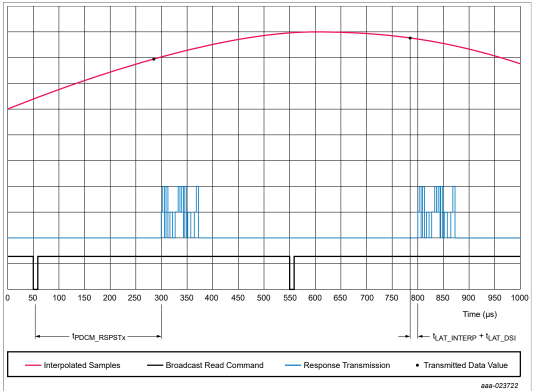
Figure 44. Synchronous sampling mode with minimum latency
