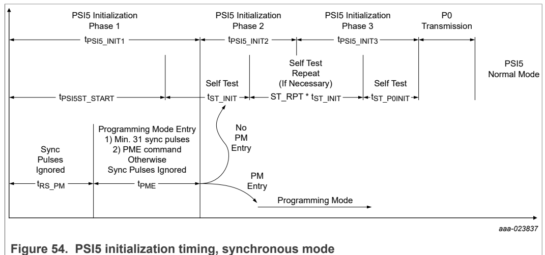
Figure 54. PSI5 initialization timing, synchronous mode
