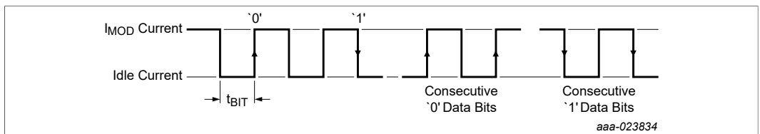
Figure 51. Manchester data bit encoding
