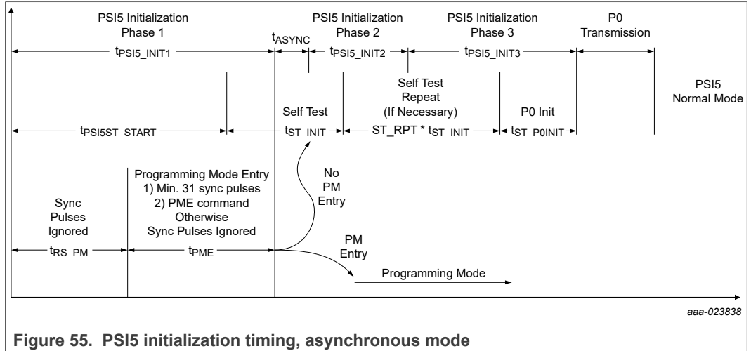
Figure 55. PSI5 initialization timing, asynchronous mode
