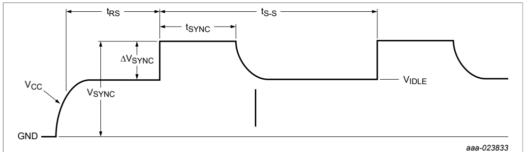
Figure 50. Sync pulse characteristics
