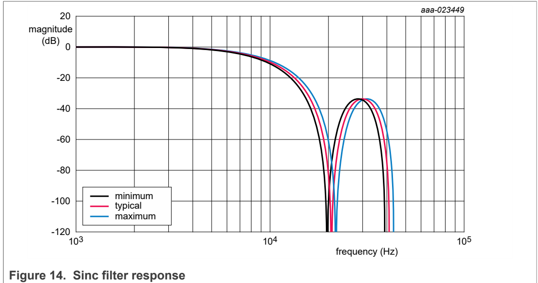
Figure 14. Sinc filter response
