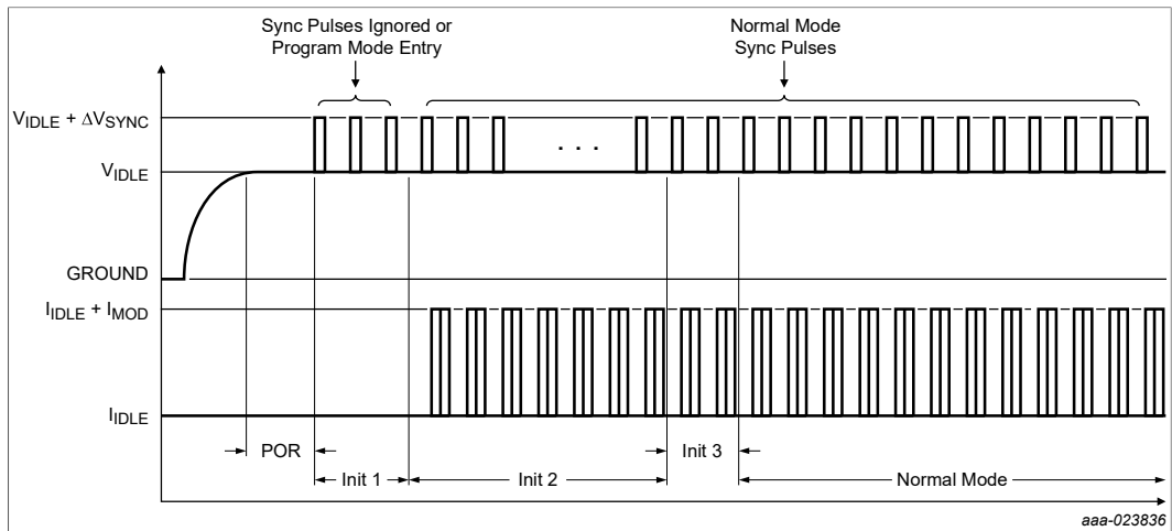
Figure 53. PSI5 sensor 10-bit initialization
