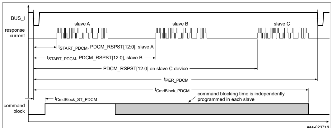
Figure 10. PSI5 oscillator training timing diagram
