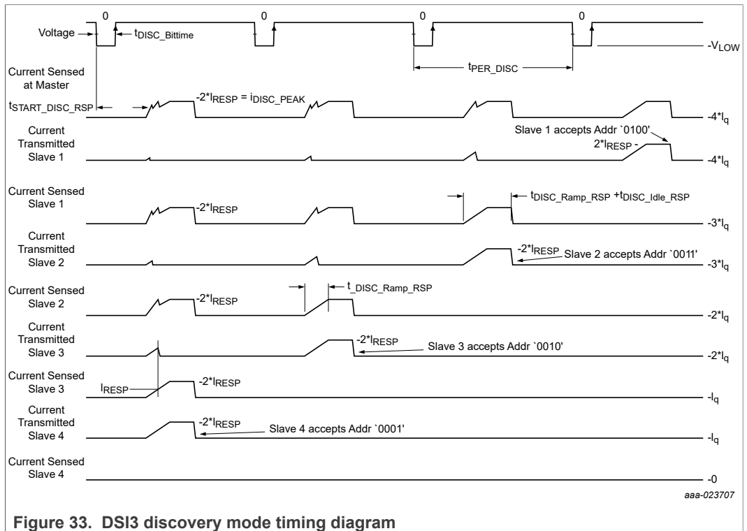
Figure 33. DSI3 discovery mode timing diagram
