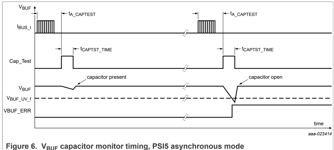
Figure 6. V_{BUF} capacitor monitor timing, PSI5 asynchronous mode
