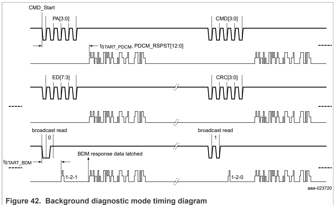
Figure 42. Background diagnostic mode timing diagram
