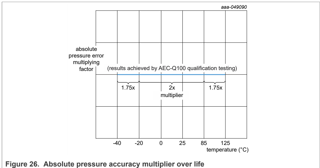
Figure 26. Absolute pressure accuracy multiplier over life
