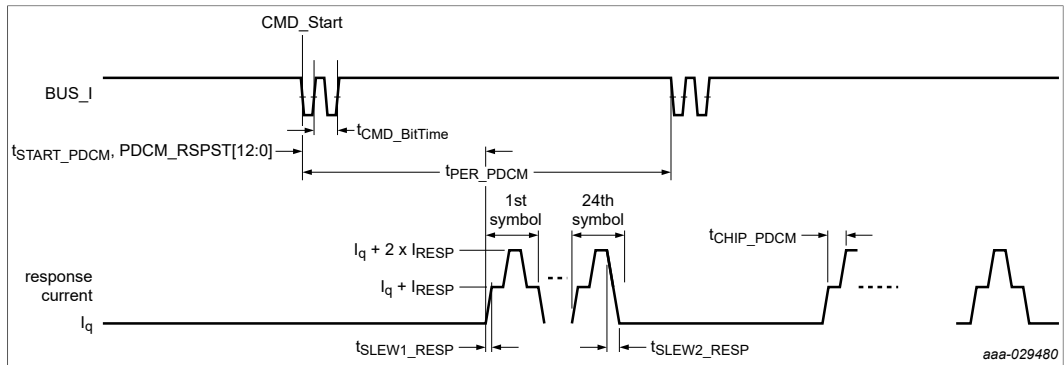
Figure 41. Periodic data collection mode timing diagram
