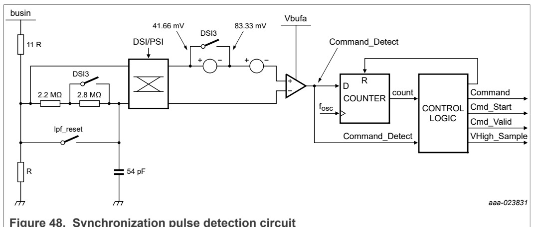
Figure 48. Synchronization pulse detection circuit
