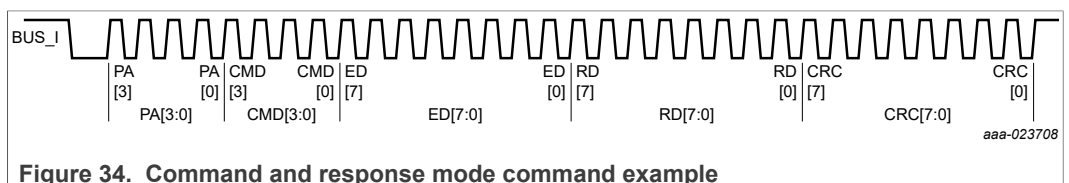
Figure 34. Command and response mode command example
