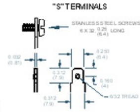
"S" TERMINALS
