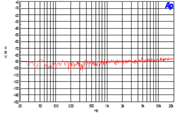
16. Noise Floor
