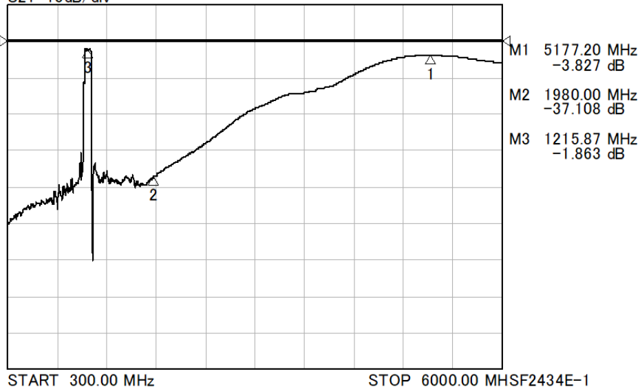
S21 10dB/div
