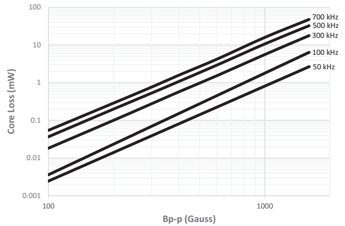
HCM1A4020V2-100-R
