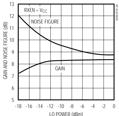
RECEIVE MIXER CONVERSION GAIN AND NOISE FIGURE vs. LO POWER
