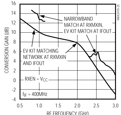
RECEIVE MIXER CONVERSION GAIN vs. RF FREQUENCY
